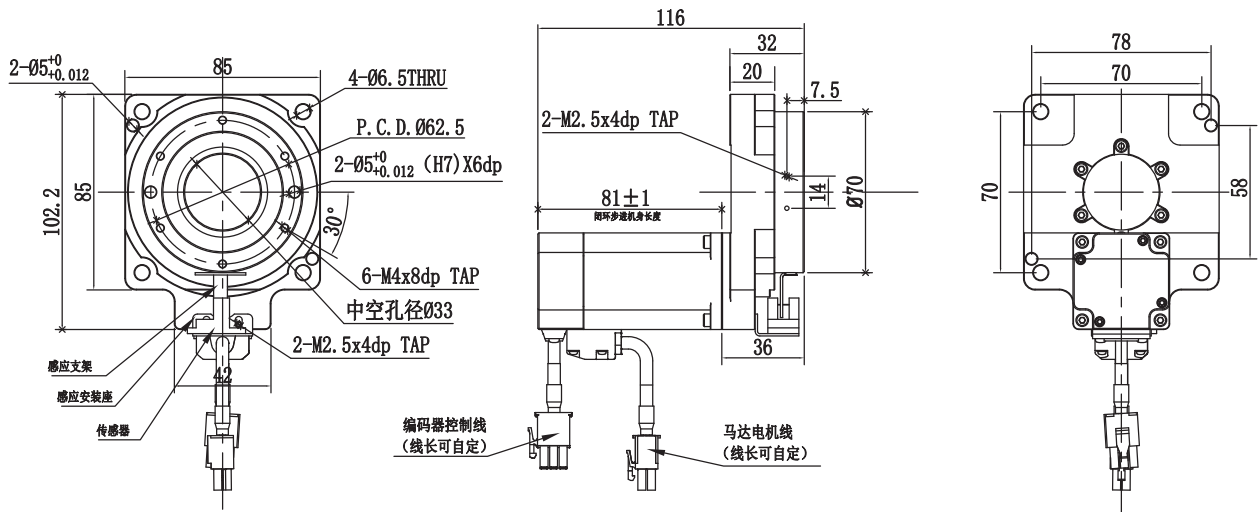
DTS085-18-STCL42 閉環步進直結式外形尺寸圖 /Closed-loop Stepping motor Dimensions
