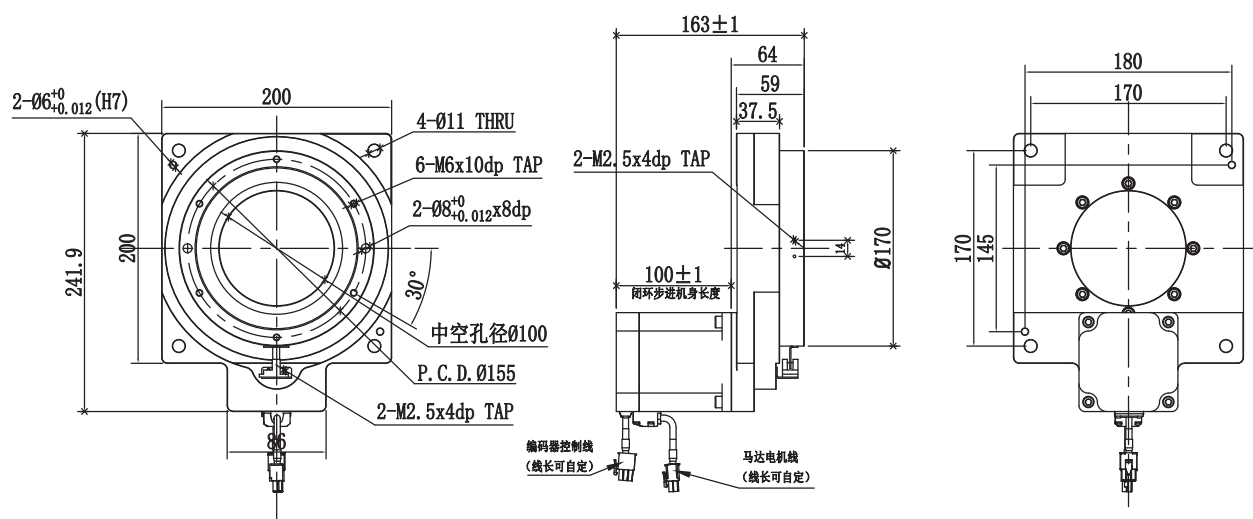
DTS200-18-STCL86 閉環步進直結式外形尺寸圖 /Closed-loop Stepping motor Dimensions
