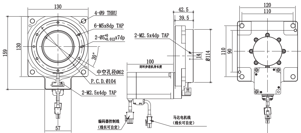
DTS130-18-STCL57 閉環步進直結式外形尺寸圖 /Closed-loop Stepping motor Dimensions
