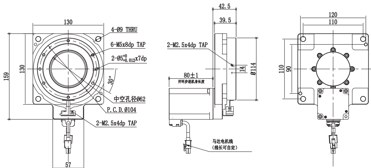
DTS130-18-ST57 開環步進直結式外形尺寸圖/Stepping motor Dimensions
