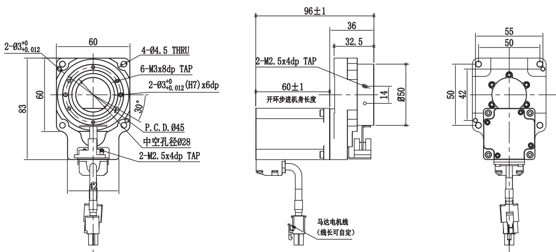
DTS085-18-ST42 開環步進直結式外形尺寸圖/Stepping motor Dimensions
