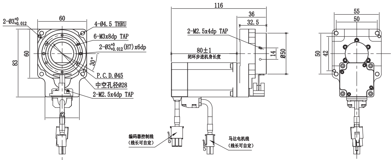
DTS060-05-STCL42 閉環步進直結式外形尺寸圖 /Closed-loop Stepping motor Dimensions
