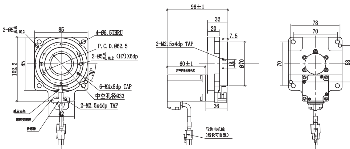
DTS085-18-ST42 開環步進直結式外形尺寸圖/Stepping motor Dimensions
