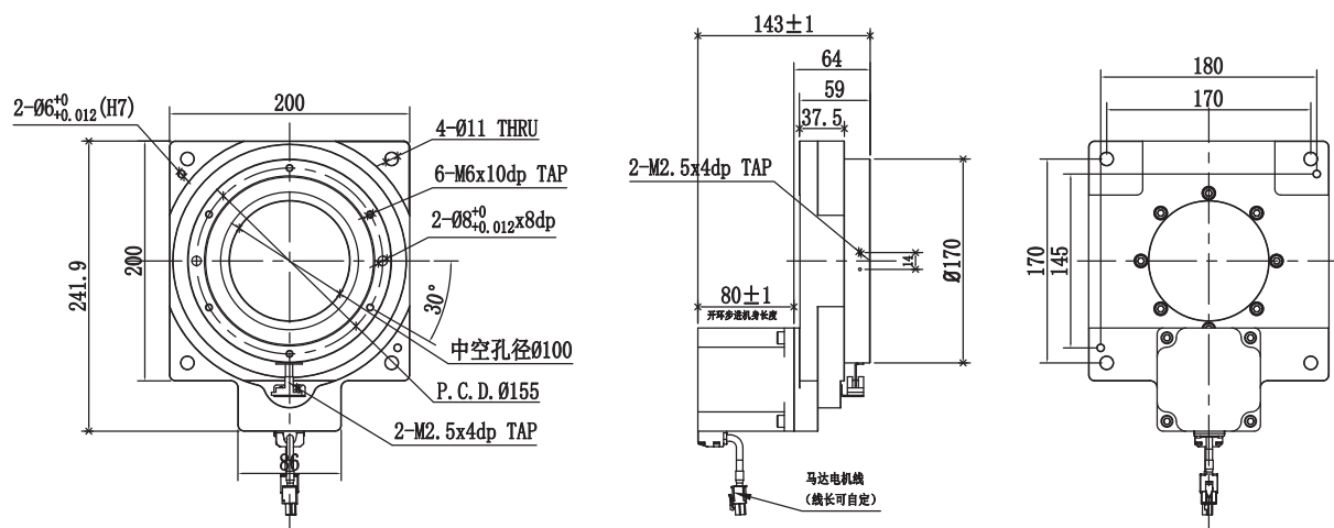
DTS200-18-ST86 開環步進直結式外形尺寸圖/Stepping motor Dimensions
