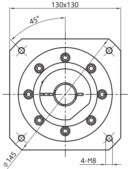
輸入端input
