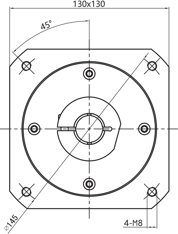
輸入端input
