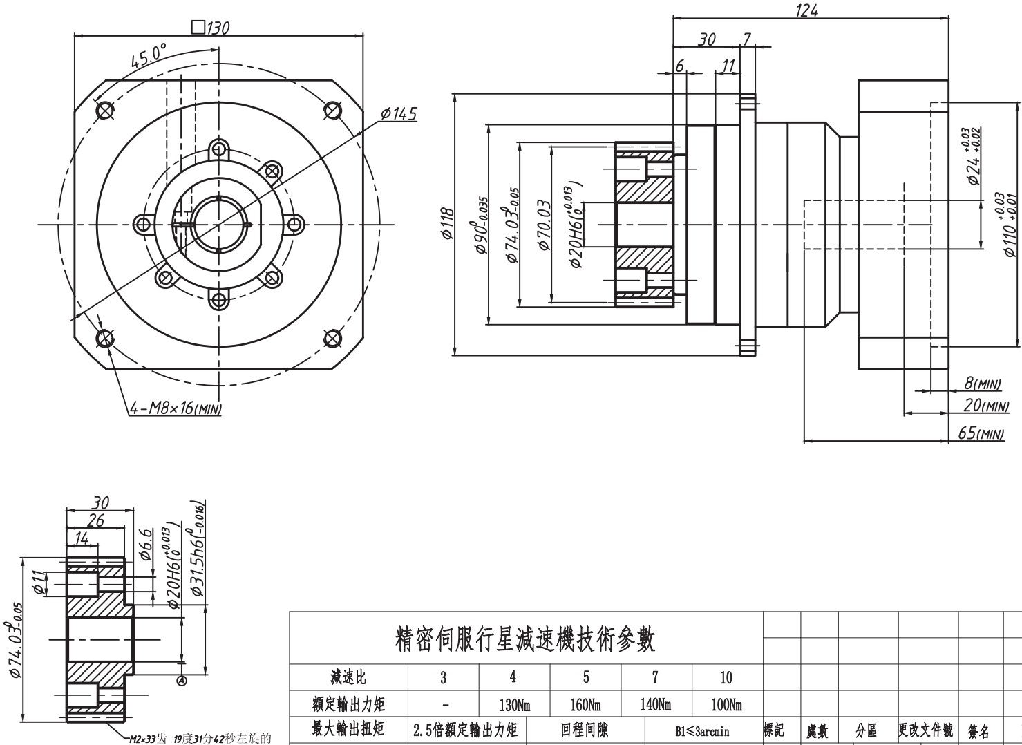
輸入端input
