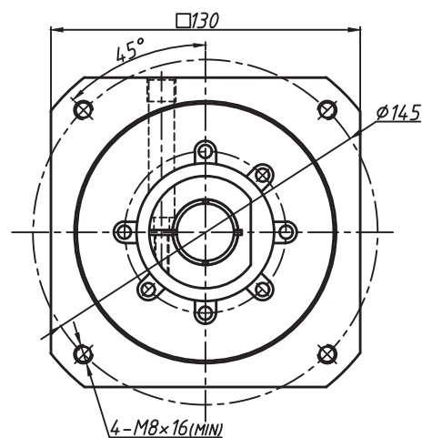
輸入端input
