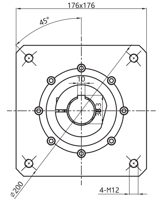
輸入端input
