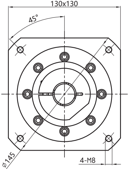
輸入端input
