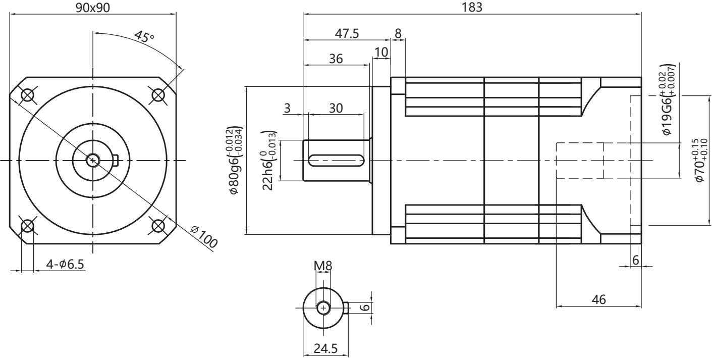
輸入端input
