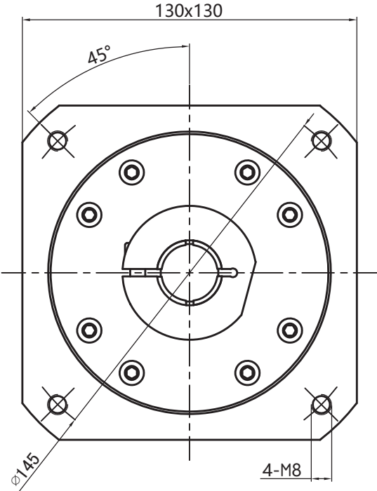
輸入端input
